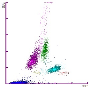
DIFF
