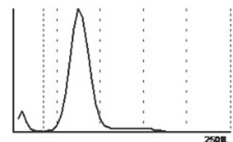
RBC
